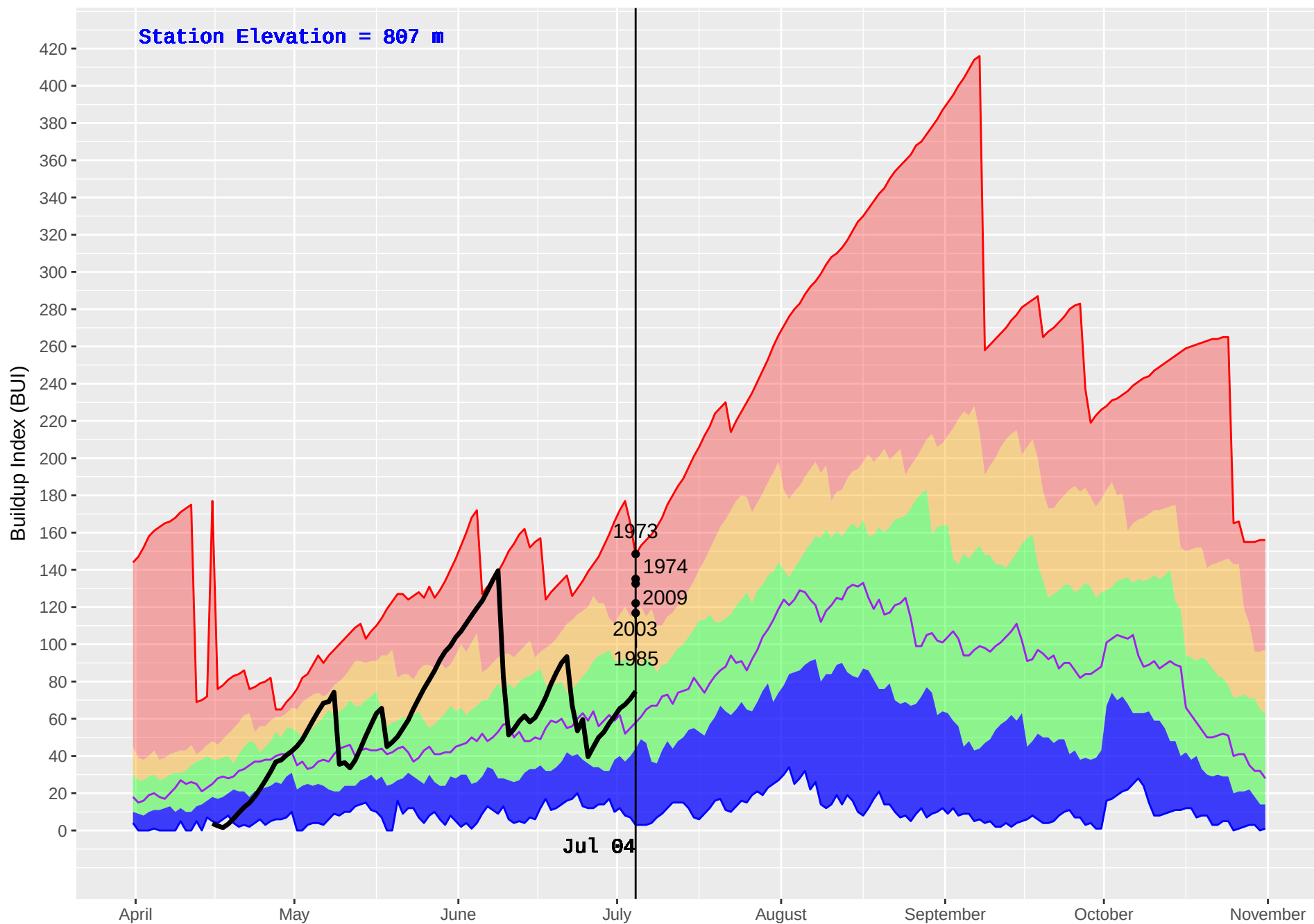
BEAVERDELL (390) : Historical (1970–2016) and Current (2018) Noon Buildup Index (BUI)
